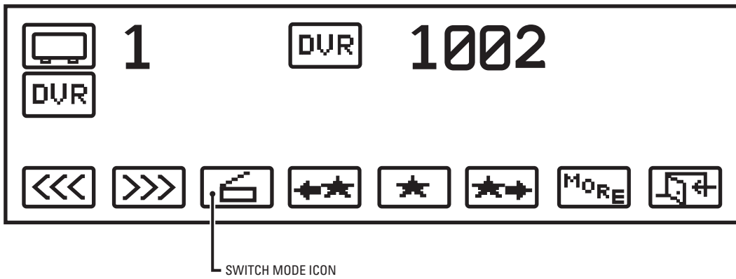
Figure 48. DVR Menu 2
